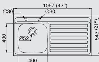
Installation drawing
