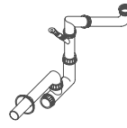
SPACE SAVER SIPHON FOR 1 BOWL DISHWASHER CONNECTION
