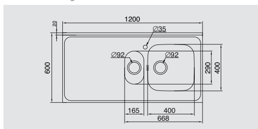
Installation drawing
