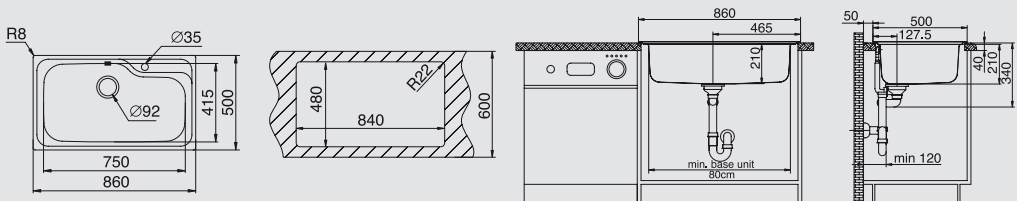
521058301 Space saver siphon
