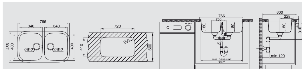
Cut out template supplied in packaging
