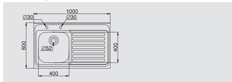
Installation drawing
